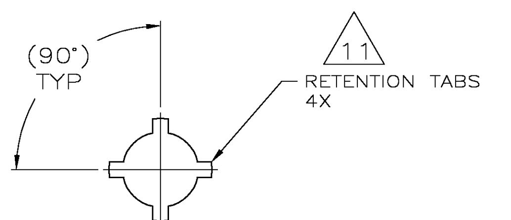
VIEW A-A SCALE 16:1
